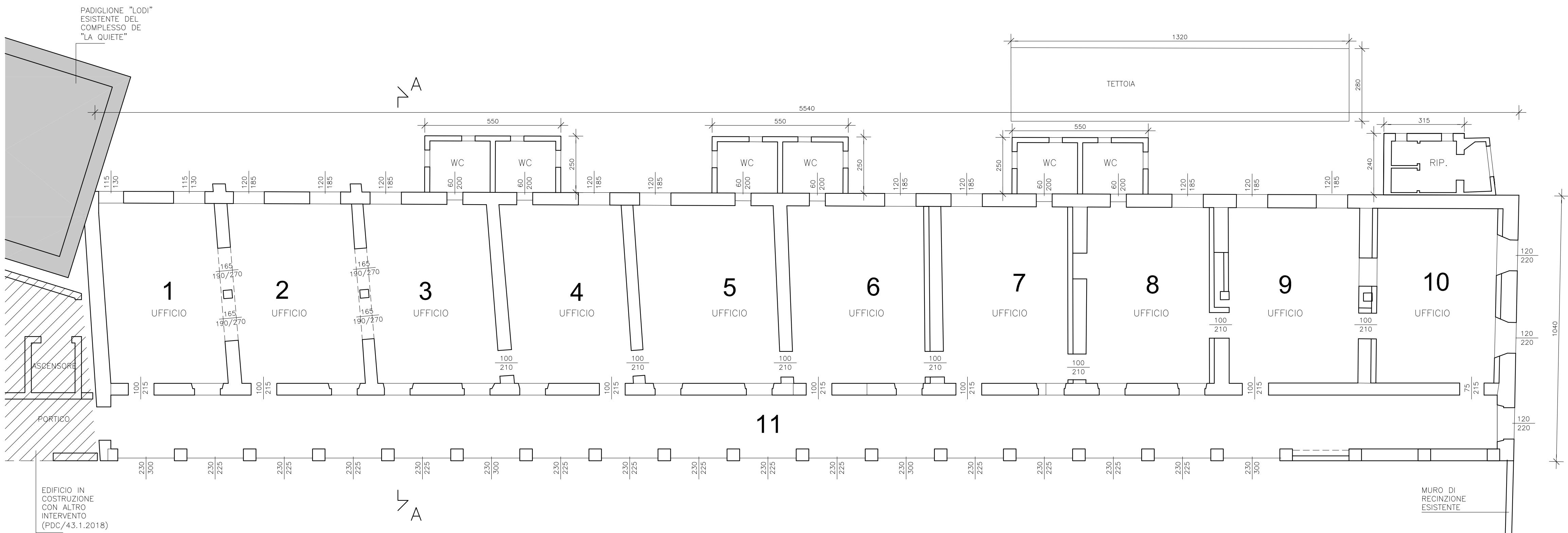
PIANO TERRA 1:100
